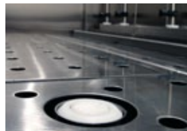
Flat floor with manifold docking.
